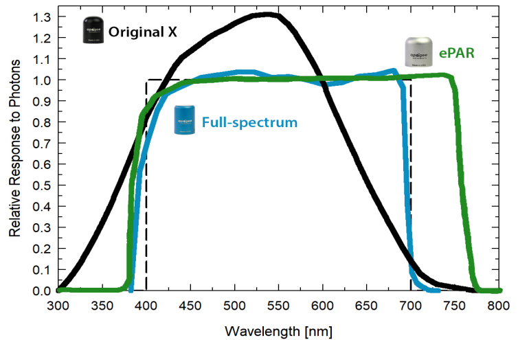
Mean spectral response measurements of six replicate Apogee MQ-210X (black), MQ-650 (green), and MQ-510 (blue) series quantum sensors compared to traditionally defined PAR 400-700 nm (dotted).
