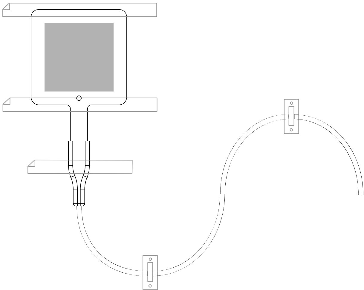
Figure 5.1.1 Installation of model FHF05-50X50 using tape to fixate the sensor and the connection block. Extra strain relief on the cable is provided using cable tie mounts equipped with double sided tape as adhesive. As indicated in Table 5.1.1, tapes fixating the sensor are preferably taped over the passive guard area and not on the sensing area (the latter indicated by grey shading in Figure 5.1.1). Please note the dot is visible in this image; this indicates that we are viewing the front side and that the other side, the back side, is attached on the object on which the sensor is mounted, as explained in Chapter 2.
